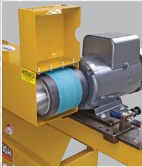
Grinding station
