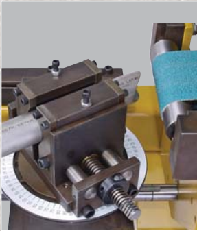
Centering vise
